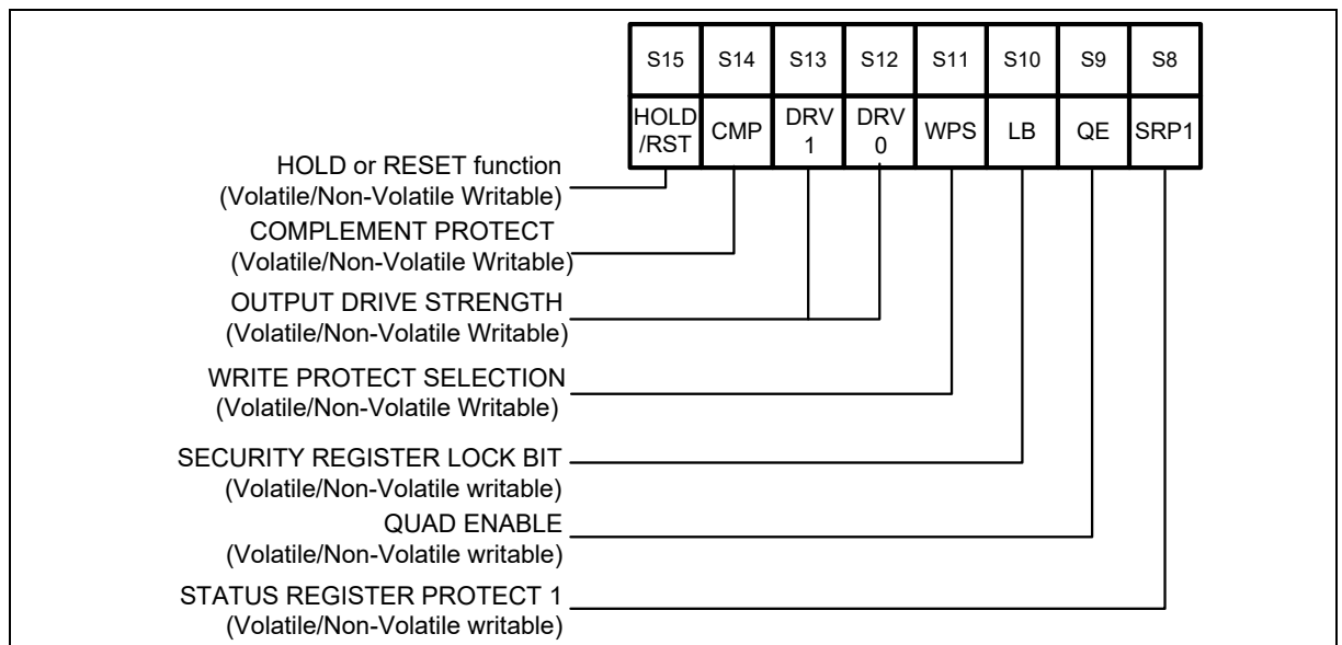
Figure 8 Status Register-2
