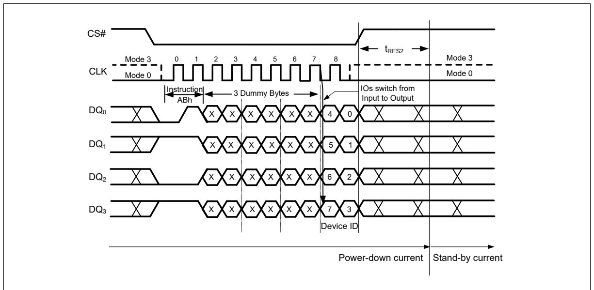
Figure 54 Release Power-down / Device ID Instruction (QPI Mode)
