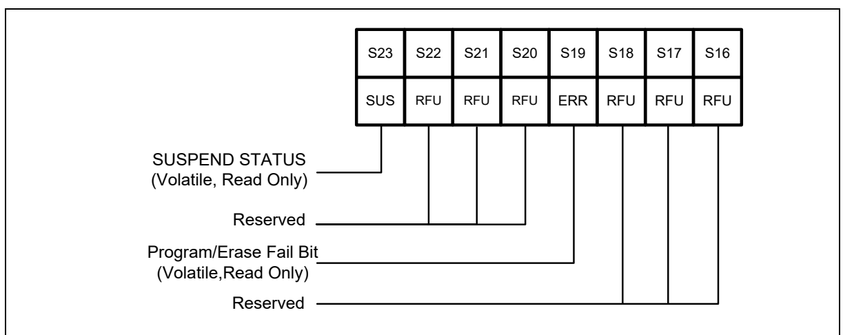
Figure 9 Status Register-3
