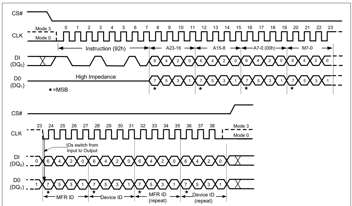
Figure 57 Read Manufacturer / Device ID Dual I/O Instruction (SPI Mode only)
