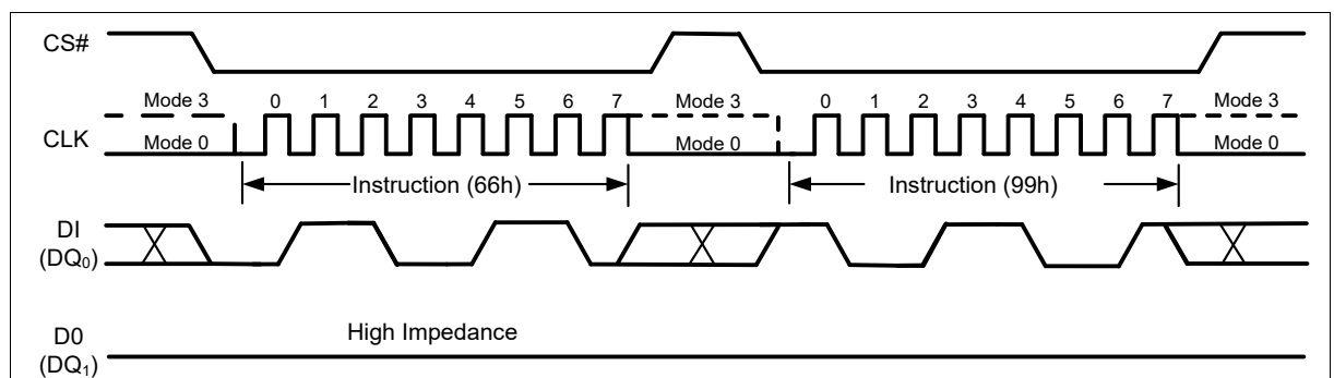
Figure 78 Enable Reset and Reset Instruction Sequence (SPI Mode)
