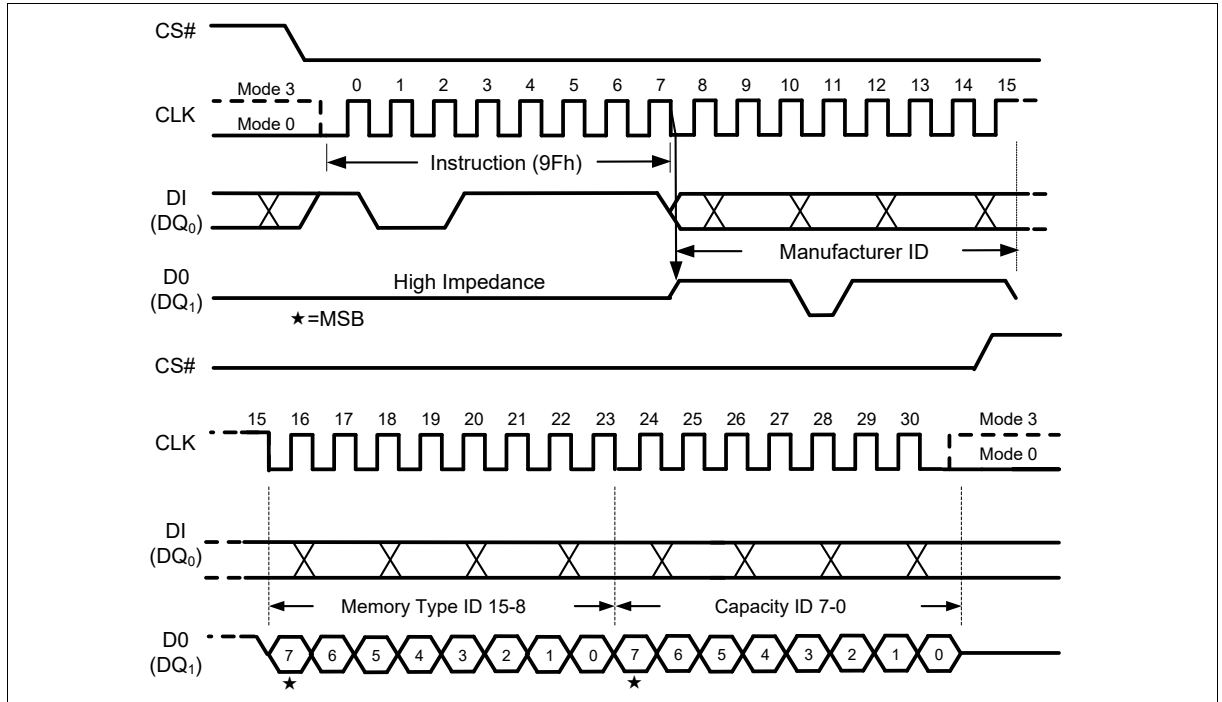
Figure 60 Read JEDEC ID Instruction (SPI Mode)
