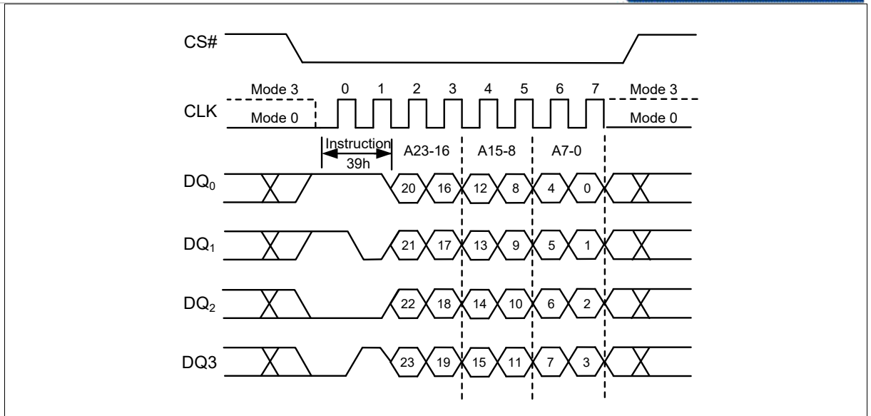
Figure 73 Individual Block/Sector Unlock Instruction (QPI Mode)
