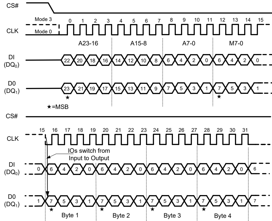
Figure 26 Fast Read Dual I/O Instruction (Previous instruction set M5-4 = 10, SPI Mode only)
