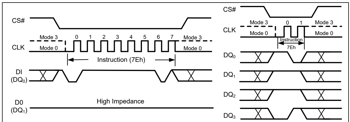
Figure 76 Global Block/Sector Lock Instruction for SPI Mode (left) or QPI Mode (right)
