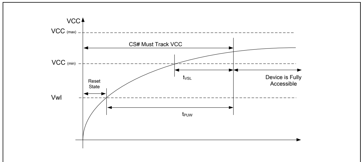
Figure 80 Power-up Timing
