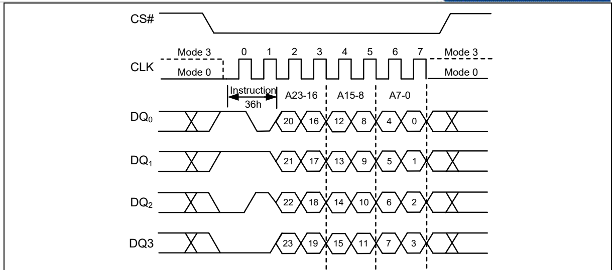
Figure 71 Individual Block/Sector Lock Instruction(QPI Mode)
