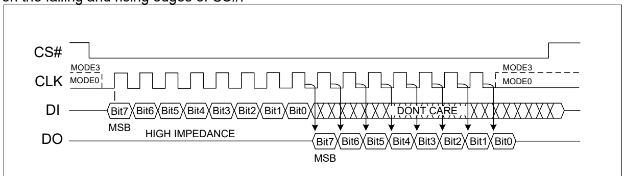
Figure 5 The difference between Mode 0 and Mode 3
