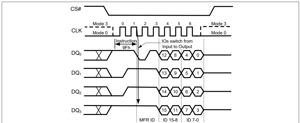
Figure 61 Read JEDEC ID Instruction (QPI Mode)
