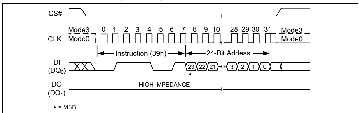
Figure 72 Individual Block/Sector Unlock Instruction (SPI Mode)
