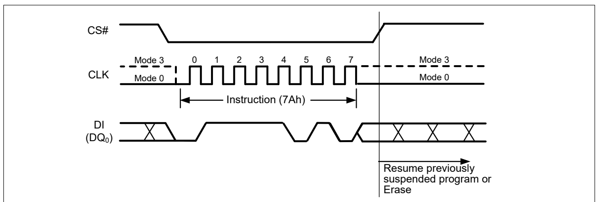
Figure 47 Erase/Program Resume Instruction (SPI Mode)
