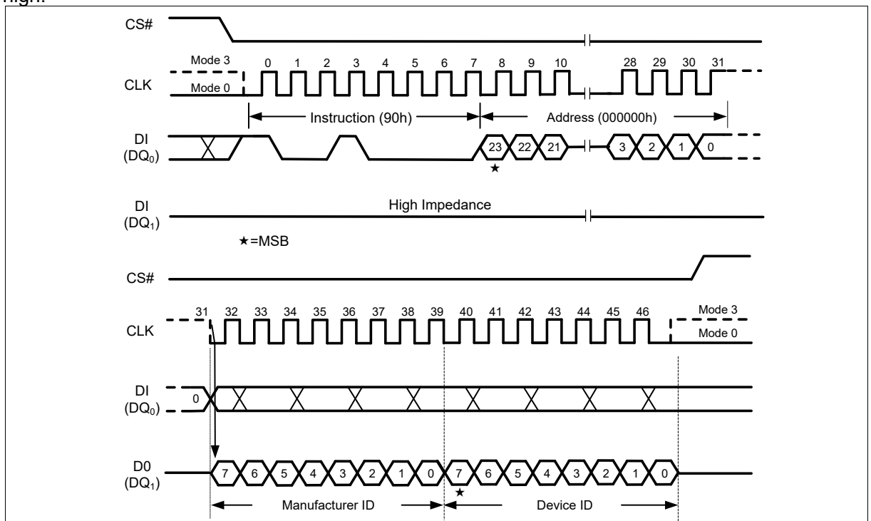
Figure 55 Read Manufacturer / Device ID Instruction (SPI Mode)
