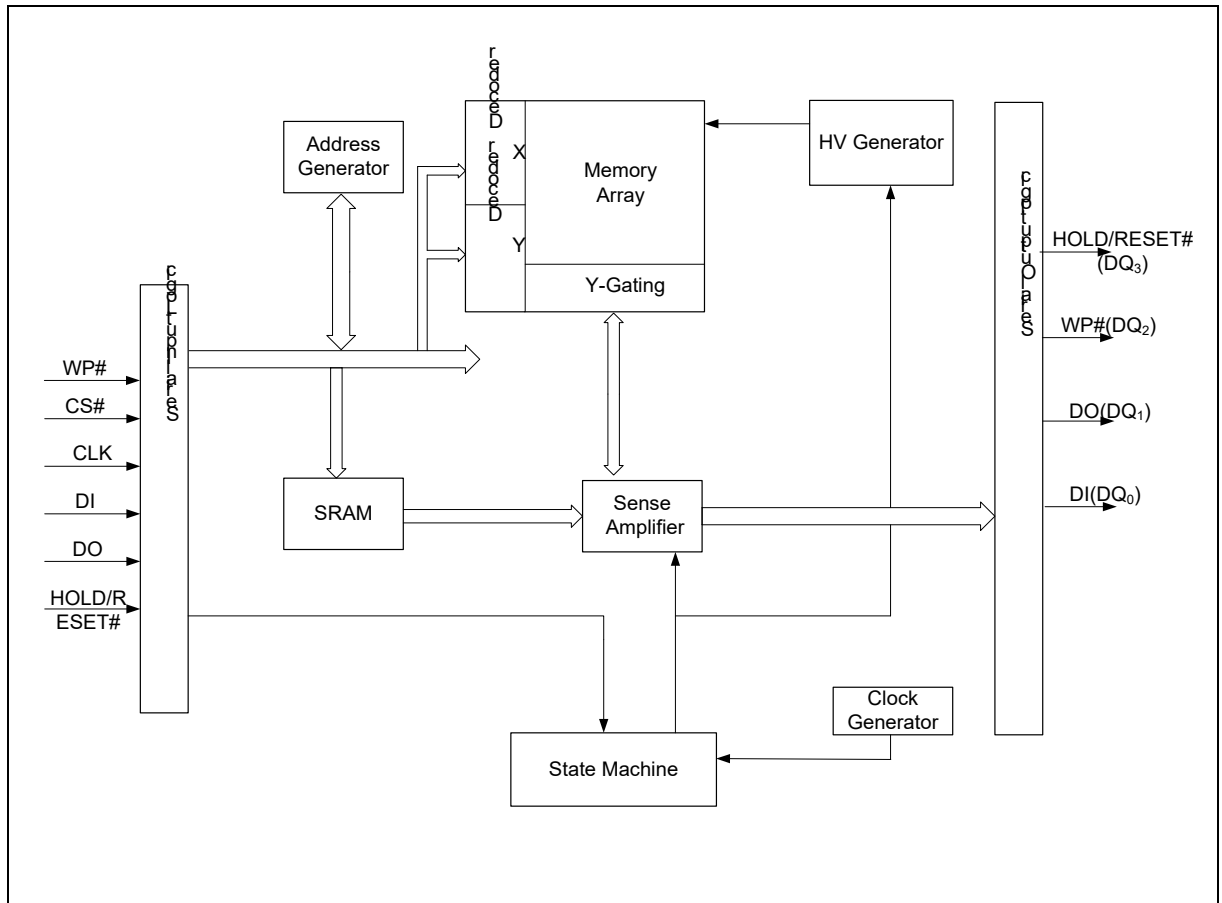
Figure 3 FM25Q128A Serial Flash Memory Block Diagram
