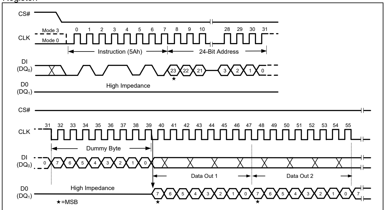
Figure 62 Read SFDP Register Instruction
