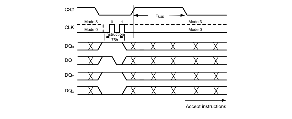
Figure 46 Erase/Program Suspend Instruction (QPI Mode)
