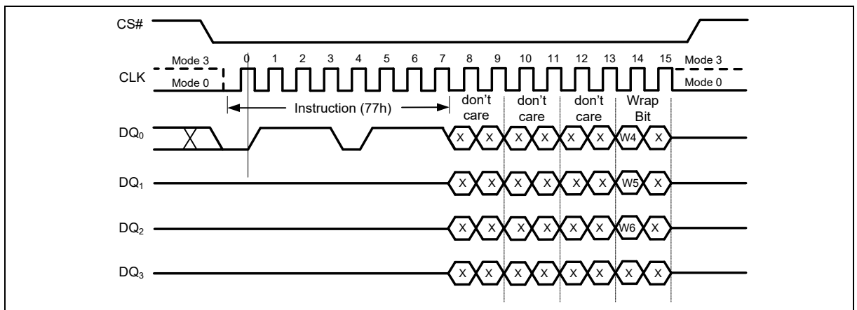
Figure 34 Set Burst with Wrap Instruction for SPI Mode
