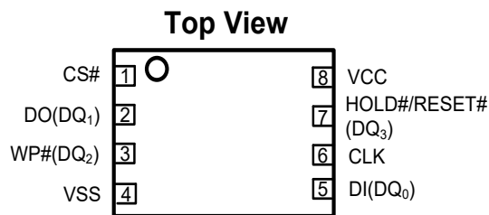
Figure 2 FM25Q128A pad assignments, 8-pad TDFN(6x5mm)
