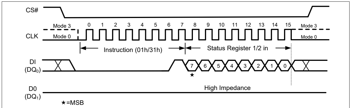
Figure 16 Write Status Register-1/2 Instruction (SPI Mode)
