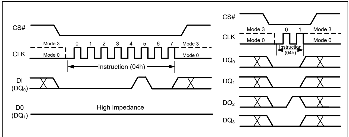
Figure 13 Write Disable Instruction for SPI Mode (left) or QPI Mode (right)
