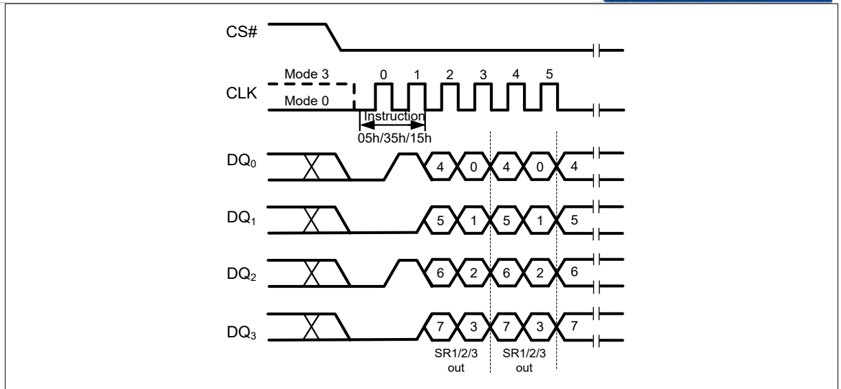
Figure 15 Read Status Register Instruction (QPI Mode)
