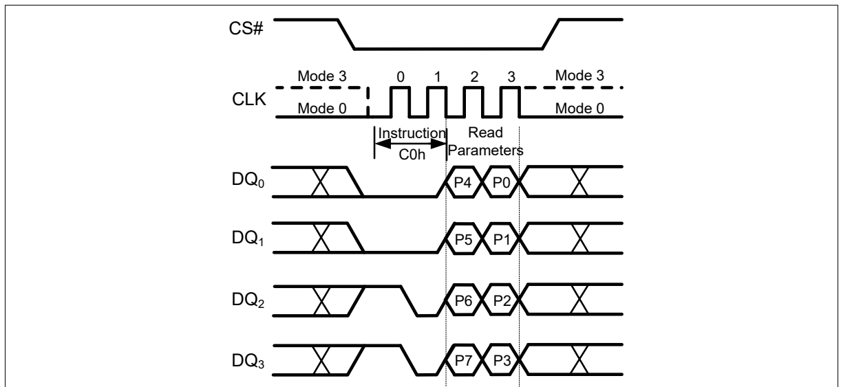
Figure 66 Set Read Parameters Instruction (QPI Mode only)
