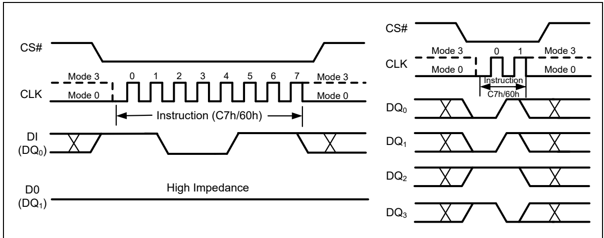
Figure 44 Chip Erase Instruction for SPI Mode (left) or QPI Mode (right)
