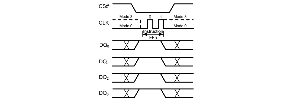
Figure 69 Disable QPI Instruction (QPI Mode only)
