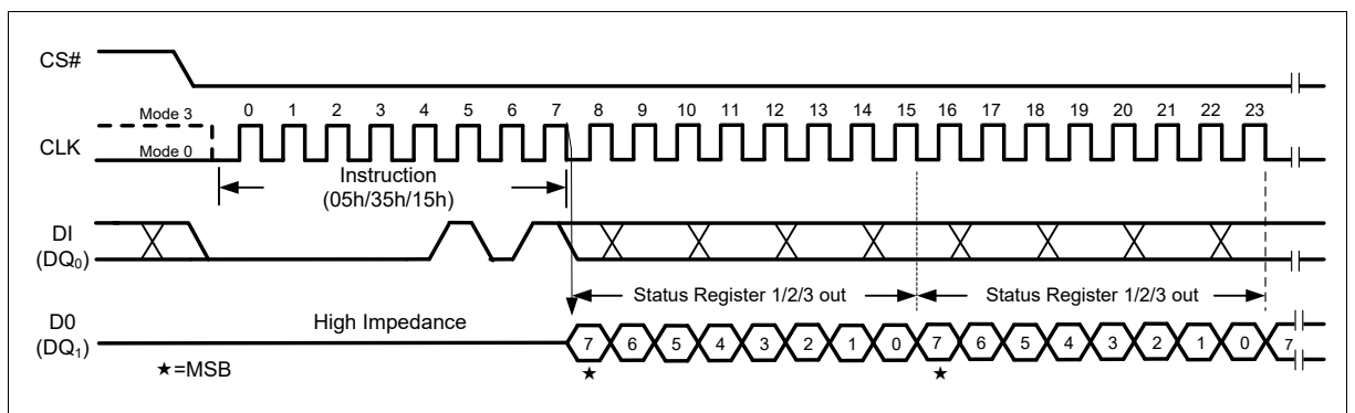
Figure 14 Read Status Register Instruction (SPI Mode)
