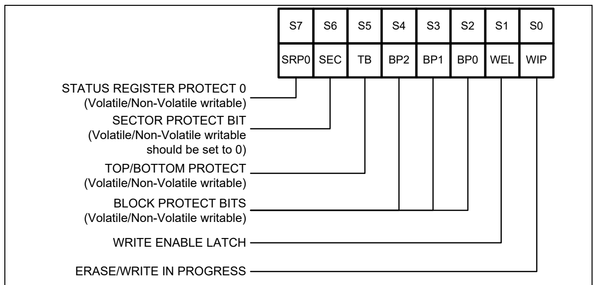
Figure 7 Status Register-1
