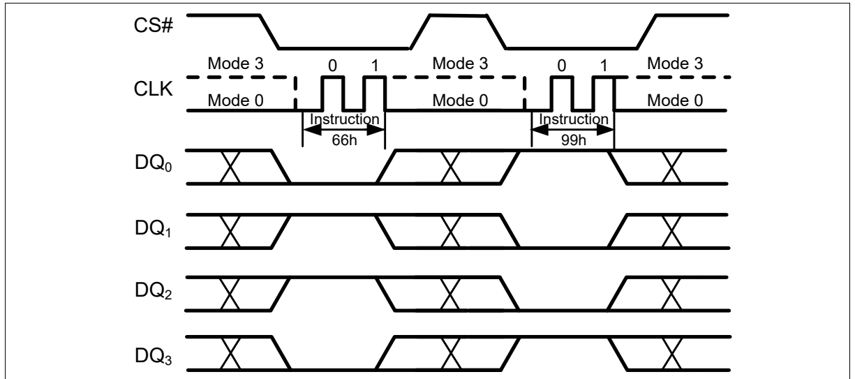
Figure 79 Enable Reset and Reset Instruction Sequence (QPI Mode)
