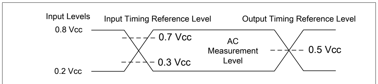
Figure 81 AC Measurement I/O Waveform
