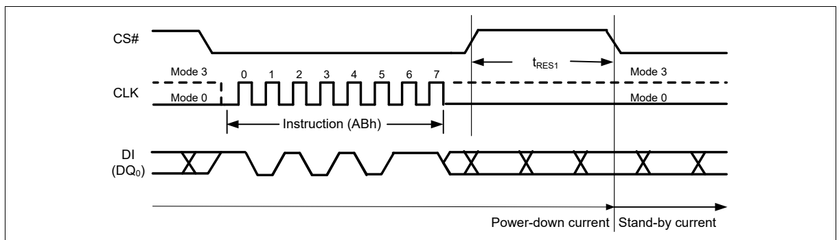
Figure 51 Release Power-down Instruction (SPI Mode)
