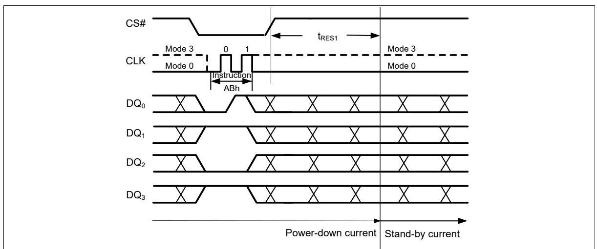
Figure 52 Release Power-down Instruction (QPI Mode)
