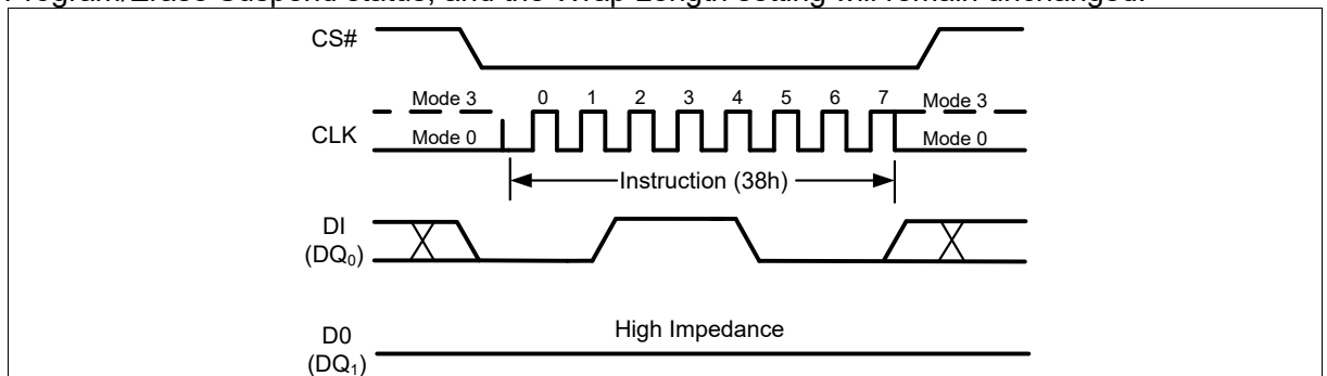
Figure 68 Enable QPI Instruction (SPI Mode only)
