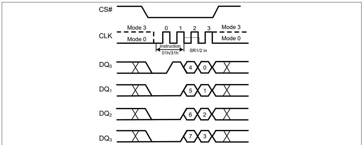
Figure 17 Write Status Register-1/2 Instruction (QPI Mode)
