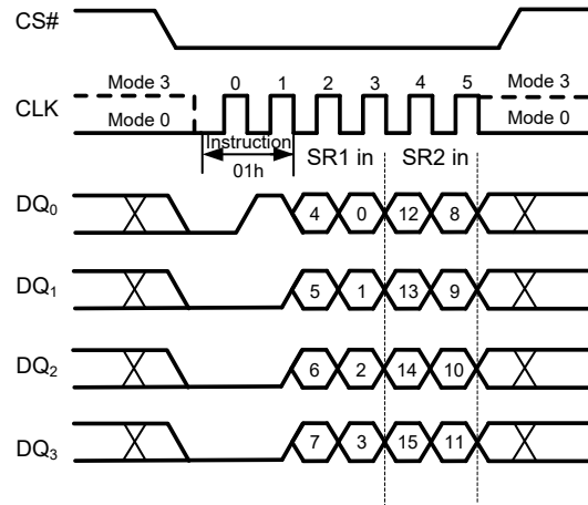
Figure 19 Write Status Register-1/2 Instruction (backward compatible,QPI Mode)
