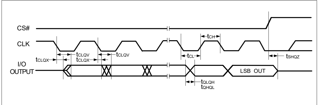
Figure 82 Serial Output Timing
