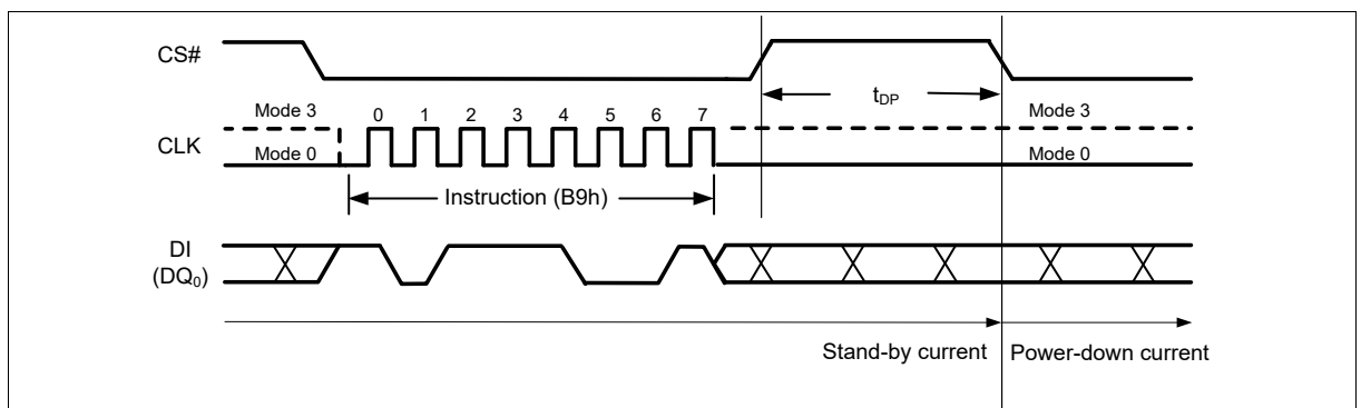
Figure 49 Deep Power-down Instruction (SPI Mode)
