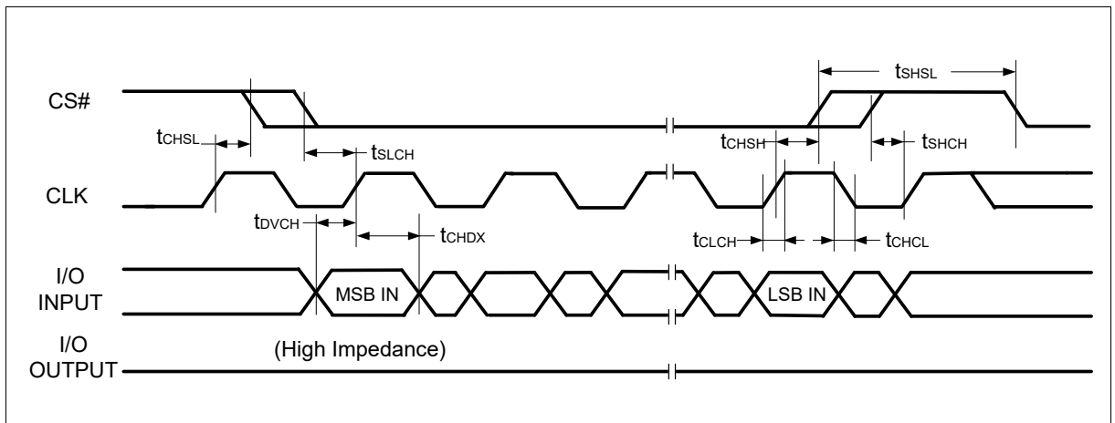
Figure 83 Serial Input Timing
