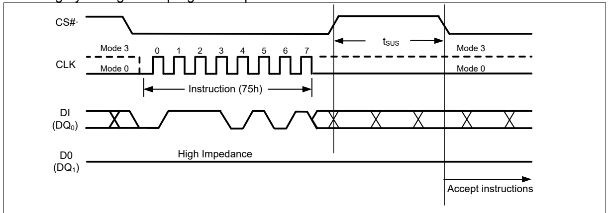
Figure 45 Erase/Program Suspend Instruction (SPI Mode)
