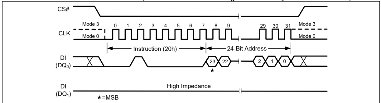
Figure 38 Sector Erase Instruction (SPI Mode)
