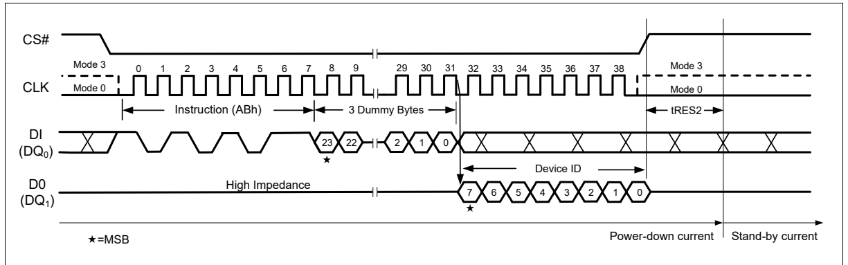
Figure 53 Release Power-down / Device ID Instruction (SPI Mode)
