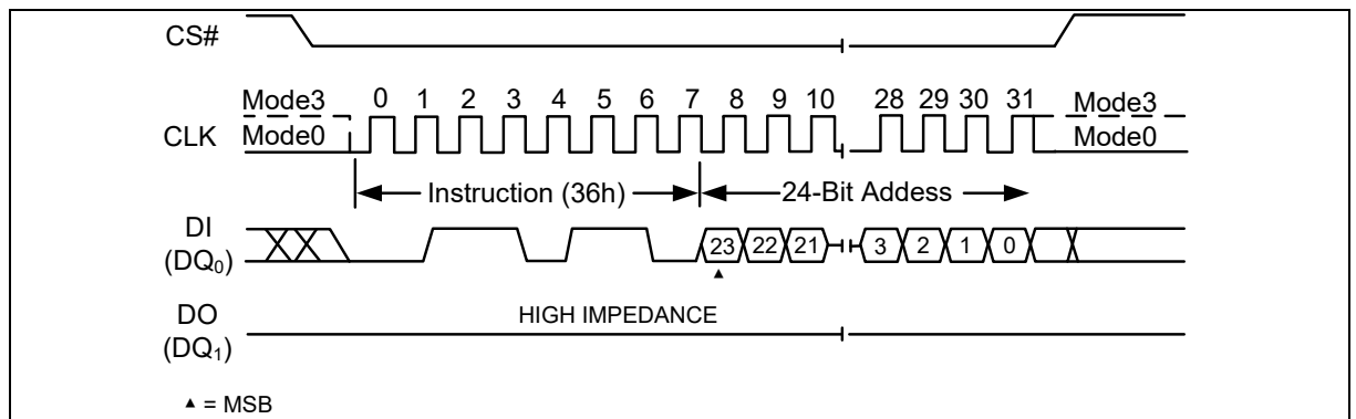
Figure 70 Individual Block/Sector Lock Instruction(SPI)
