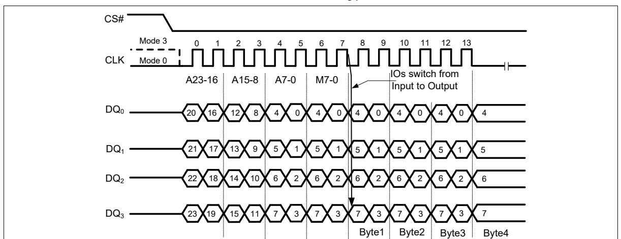
Figure 33 Octal Word Read Quad I/O Instruction (Previous instruction set M5-4 = 10, SPI Mode only)
