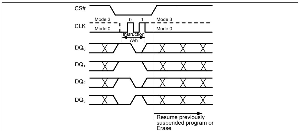
Figure 48 Erase/Program Resume Instruction (QPI Mode)
