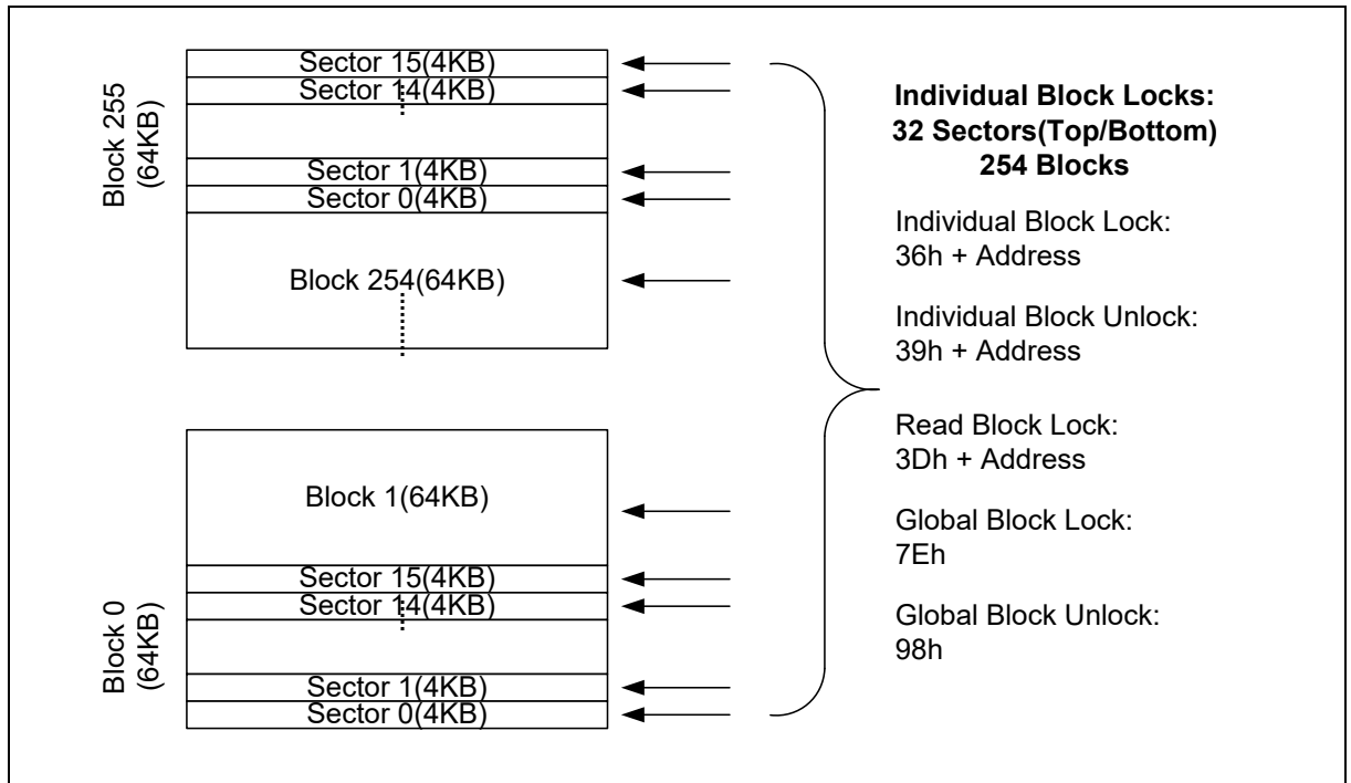
Figure 10 Individual Sector/Block Locks
