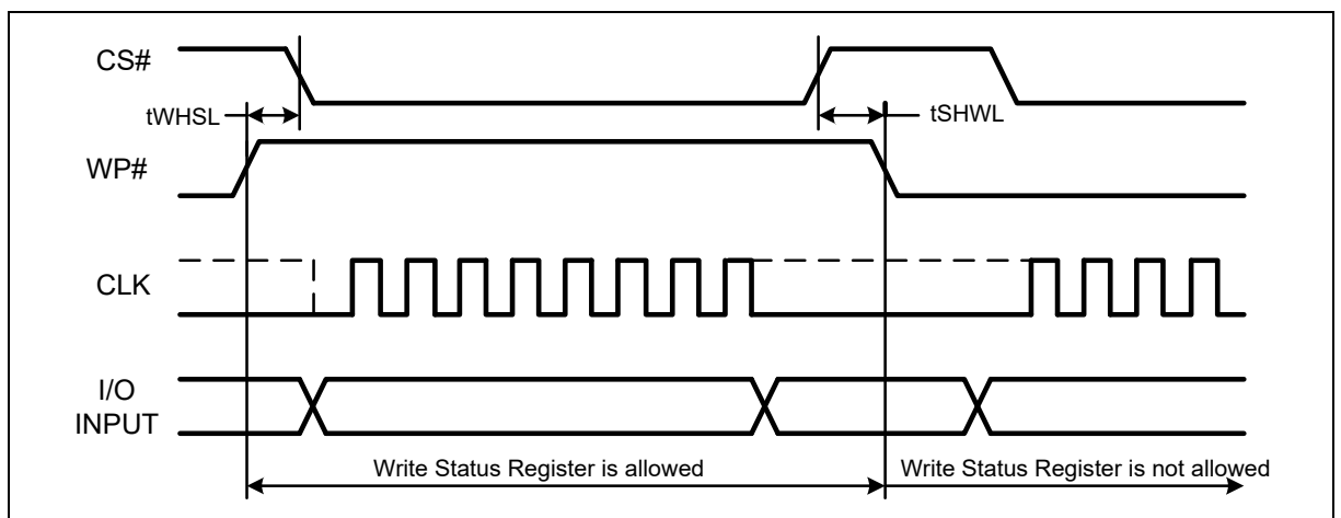
Figure 85 WP# Timing
