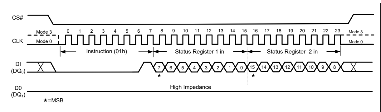
Figure 18 Write Status Register-1/2 Instruction (backward compatible, SPI Mode)
