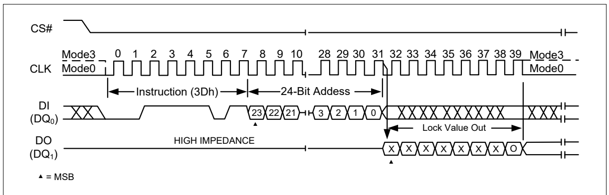
Figure 74 Read Block/Sector Lock Instruction (SPI Mode)
