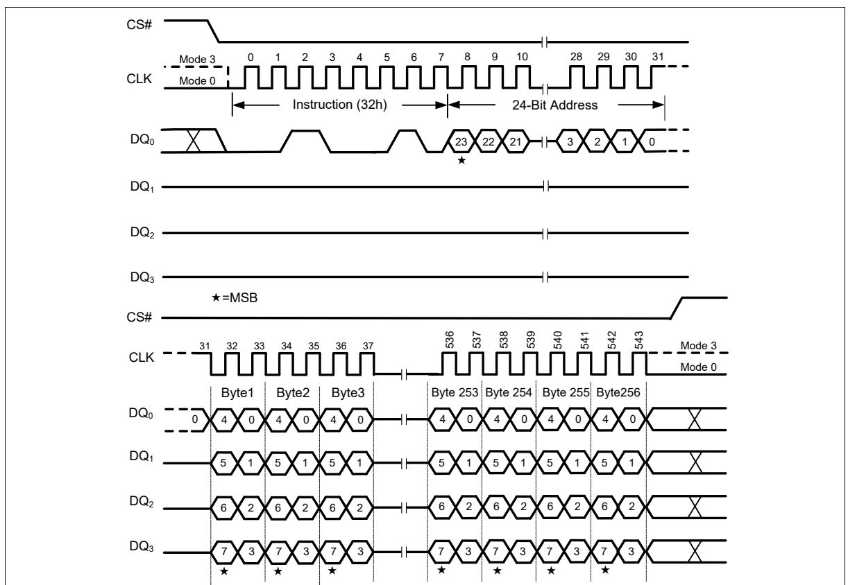
Figure 37 Quad Input Page Program Instruction (SPI Mode only)
