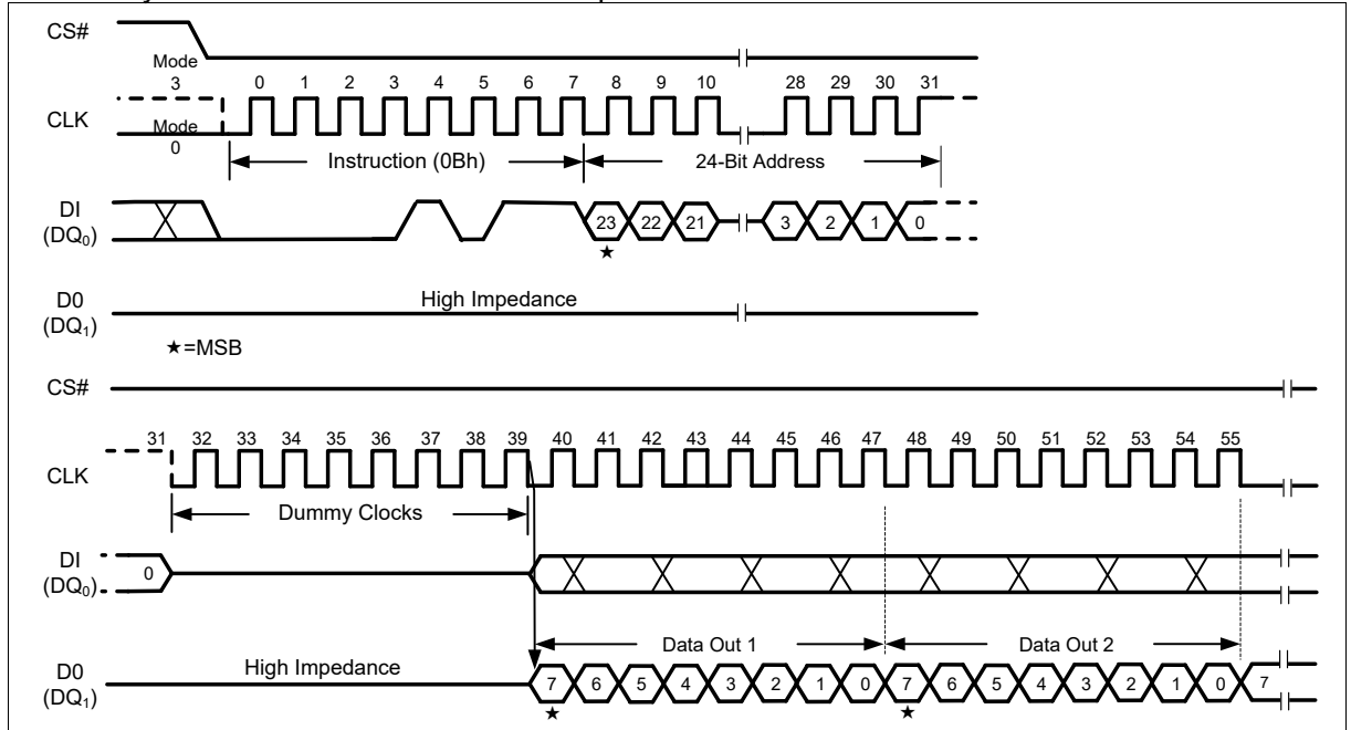
Figure 21 Fast Read Instruction (SPI Mode)
