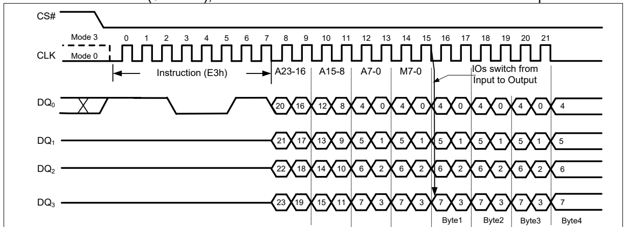
Figure 32 Octal Word Read Quad I/O Instruction (Initial instruction or previous M5-4 ≠ 10, SPI Mode only)
