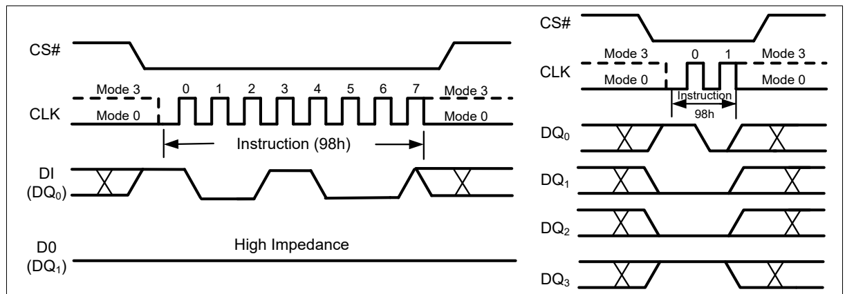
Figure 77 Global Block/Sector Unlock Instruction for SPI Mode (left) or QPI Mode (right)
