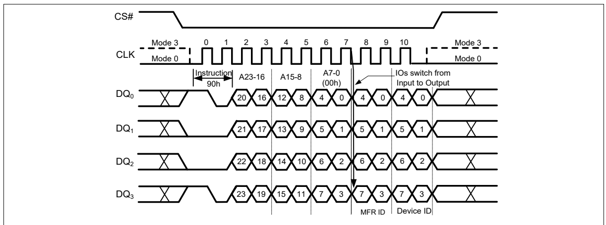
Figure 56 Read Manufacturer / Device ID Instruction (QPI Mode)
