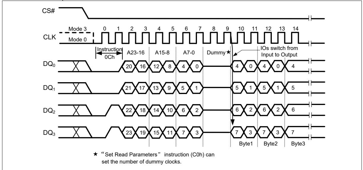
Figure 67 Burst Read with Wrap Instruction (QPI Mode only)
