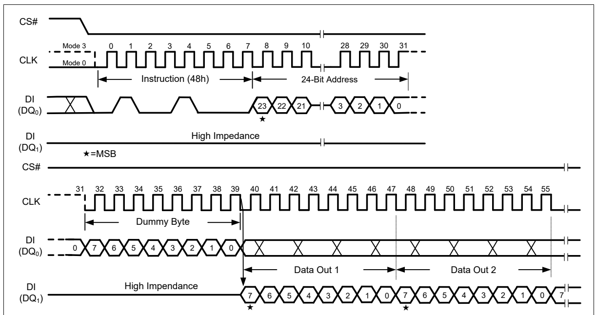
Figure 65 Read Security Sector Instruction (SPI Mode only)
