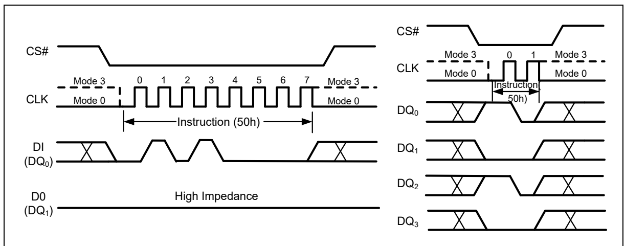
Figure 12 Write Enable for Volatile Status Register Instruction for SPI Mode (left) or QPI Mode (right)
