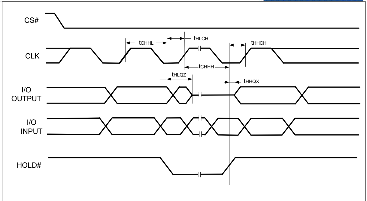
Figure 84 Hold Timing
