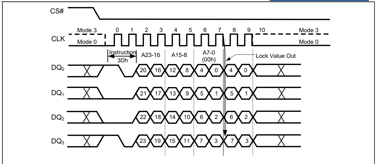
Figure 75 Read Block/Sector Lock Instruction (QPI Mode)
