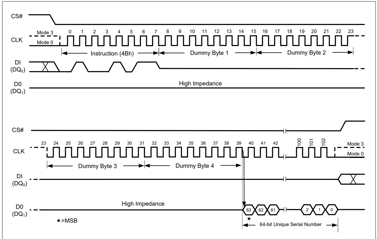
Figure 59 Read Unique ID Number Instruction (SPI Mode only)
