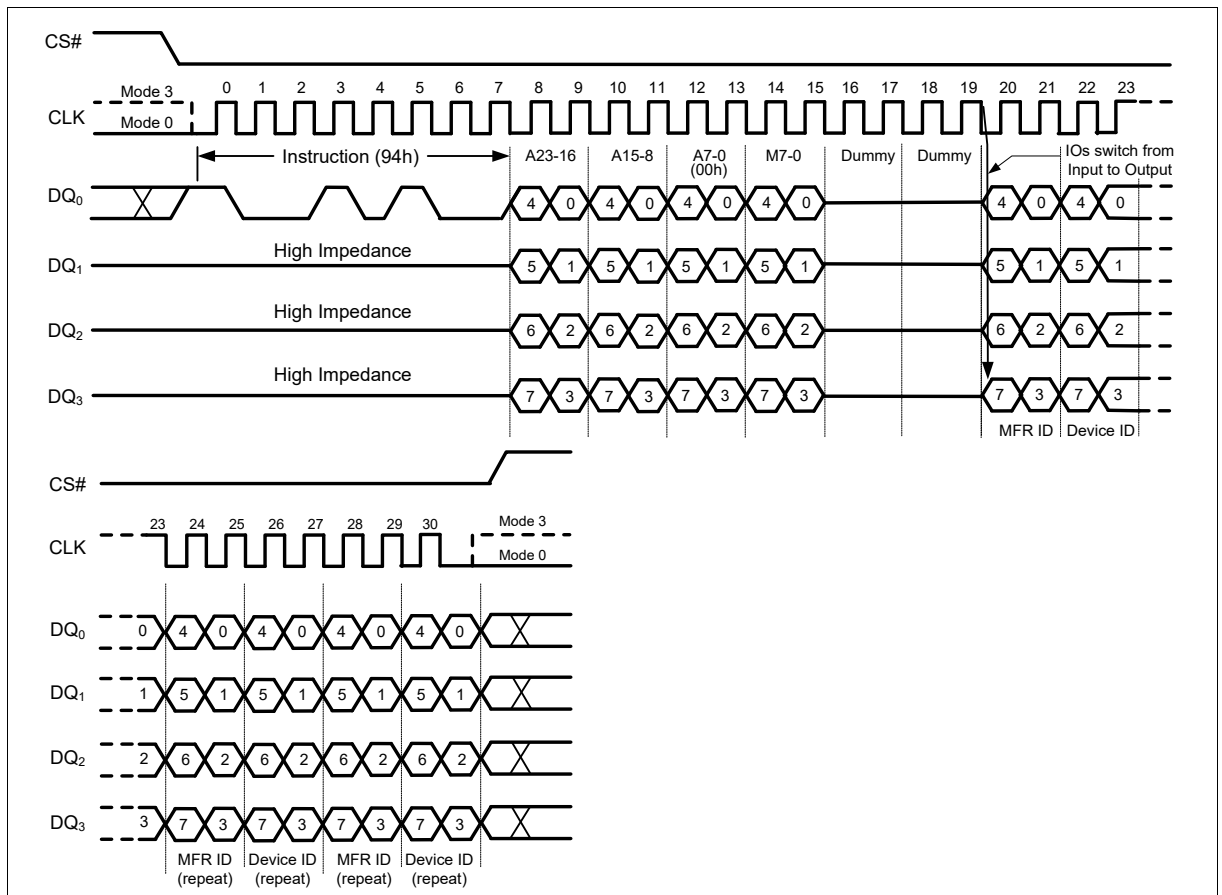
Figure 58 Read Manufacturer / Device ID Quad I/O Instruction (SPI Mode only)
