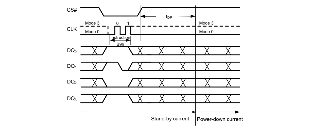
Figure 50 Deep Power-down Instruction (QPI Mode)
